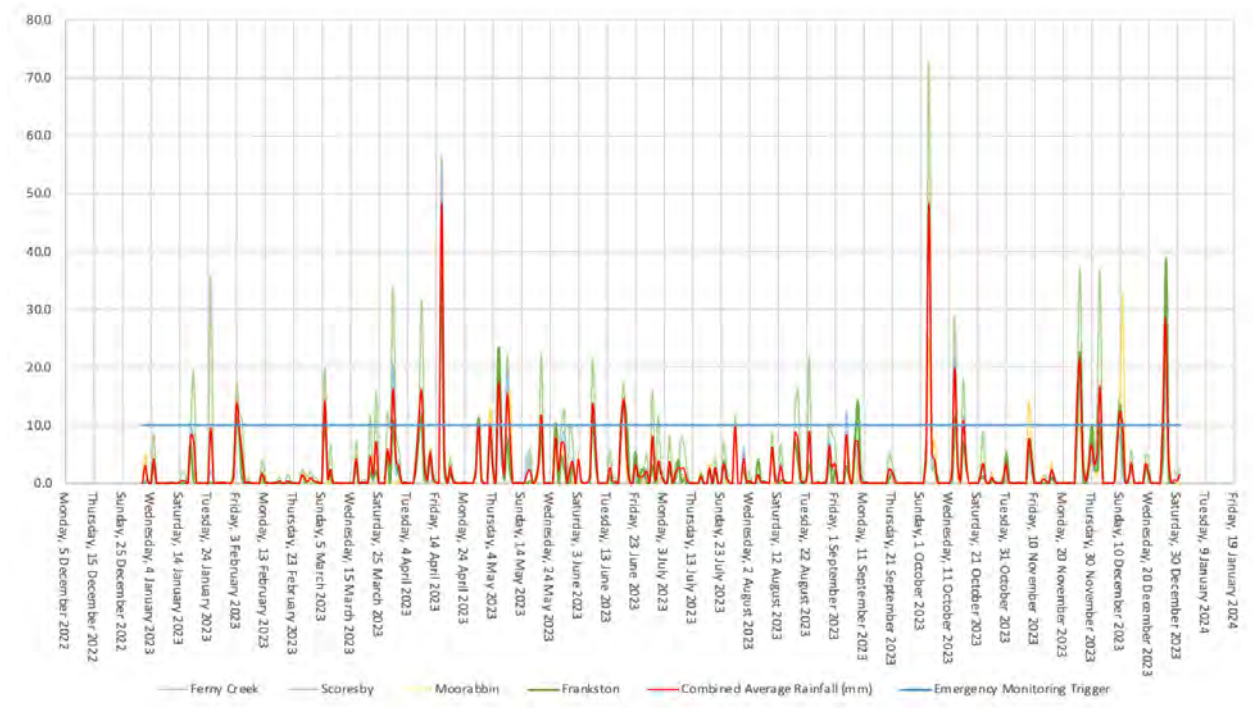
Figure 3 2023 rainfall chart
